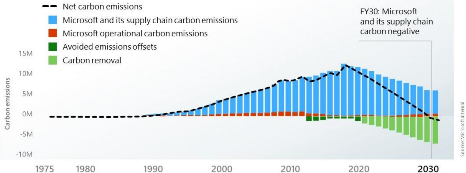
Annual carbon emissions
